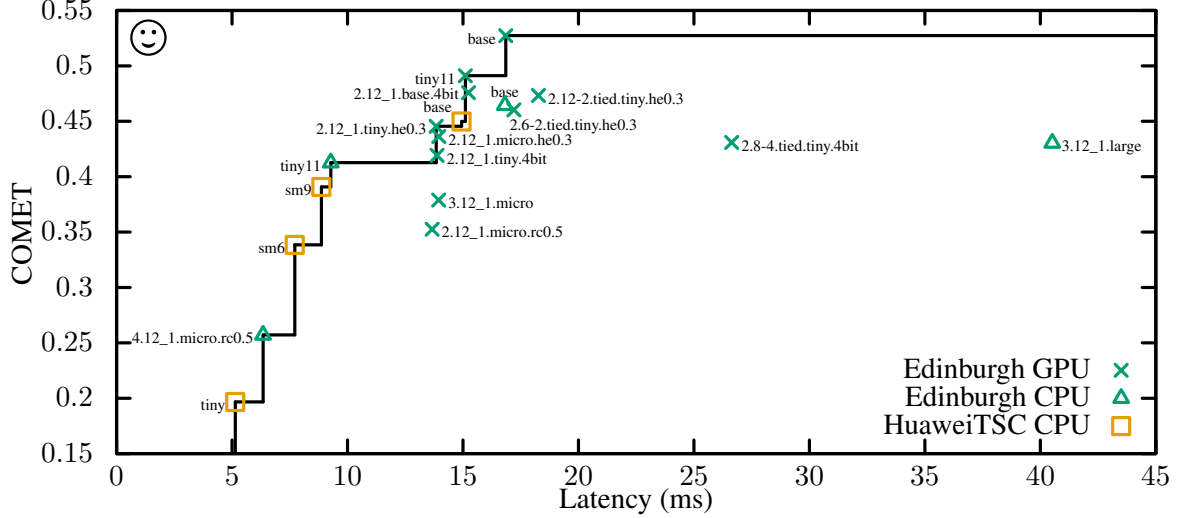
Figure 4: Latency of combined CPU and GPU systems with COMET scores. To improve the scale of the graph, low-quality variants 4.12_1.tiny.rowcol-0.5.ft8 and 4.12_1.micro.rowcol-0.5.ft8 from Edinburgh are not shown. Their respective COMET scores are -0.073 and -0.173.
