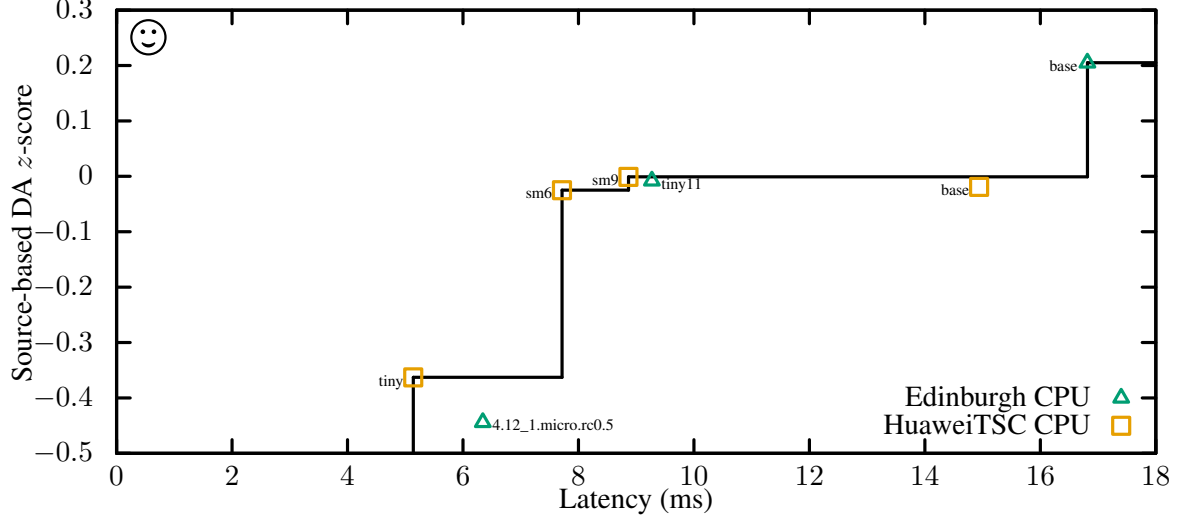
Figure 3: Latency of select CPU systems with source-based direct assessment. Contrastive direct assessment (Table 7) insignificantly ranked HuaweiTSC's base > Edinburgh's tiny11 > HuaweiTSC's sm9.
