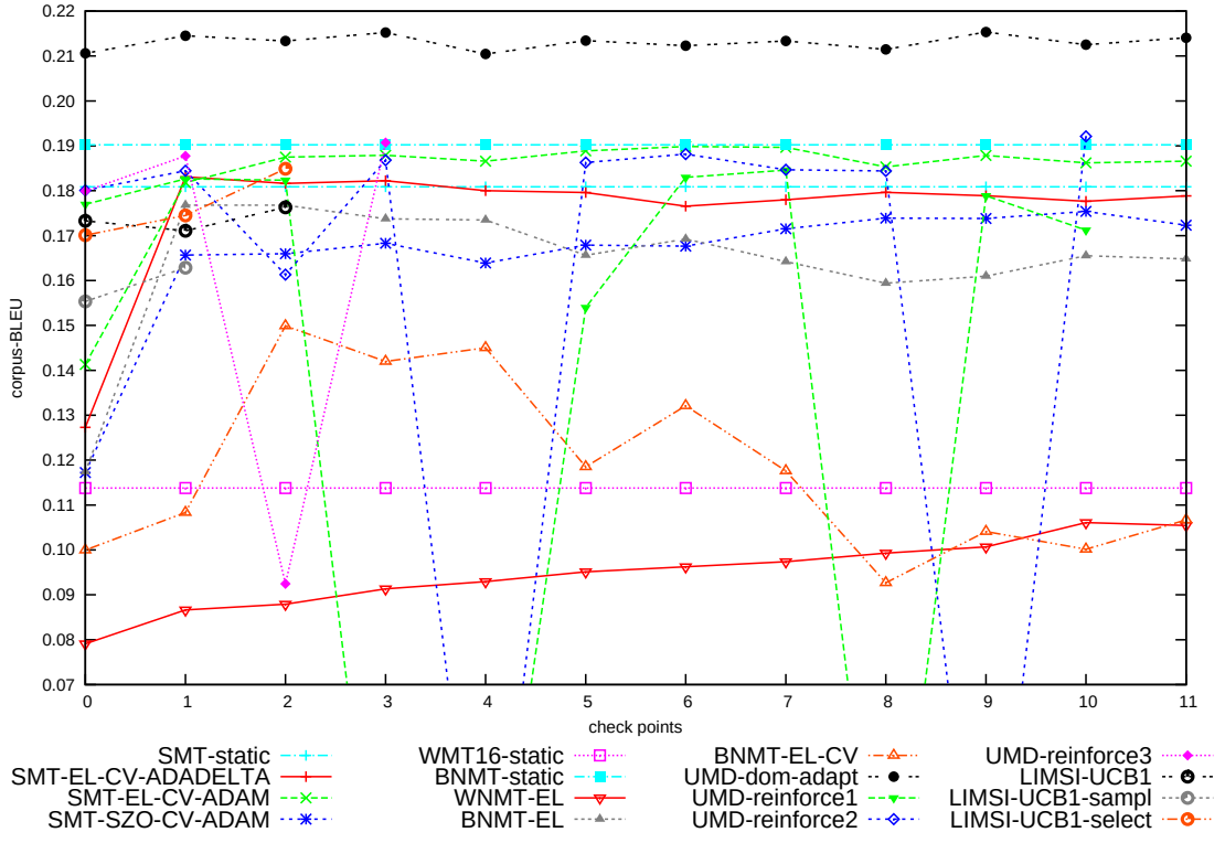
(a) corpus-BLEU
