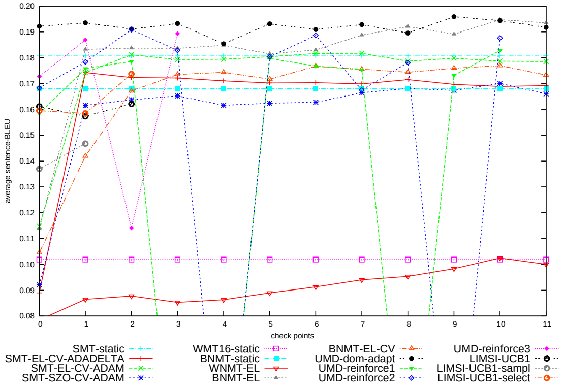
(b) sentence-BLEU
